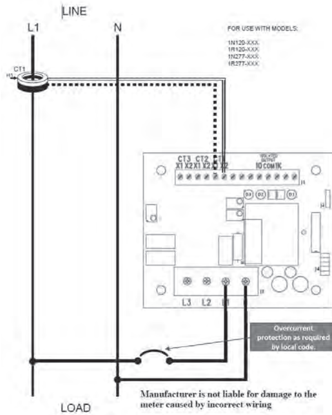
Figure 7: 1-phase, 2-wire Hookup Diagram
