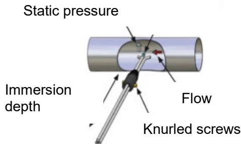
Fig. 39: Measuring the air speed with the S-tube
