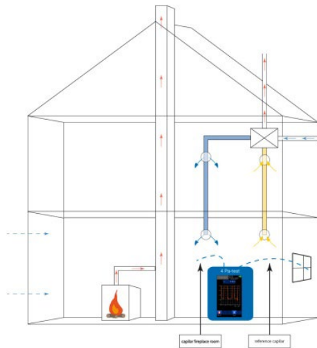
Fig. 56: Plan of the 4 Pa Test
