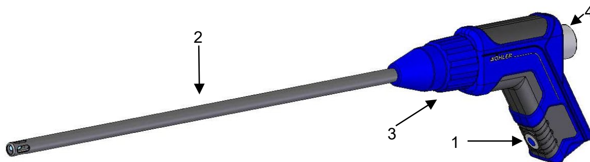
Fig. 23: Probe handle with gas probe 295 mm
