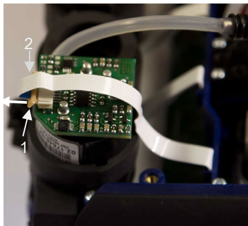
Fig. 74: Sensor with locking mechanism (1) and flexible conductor (2)
