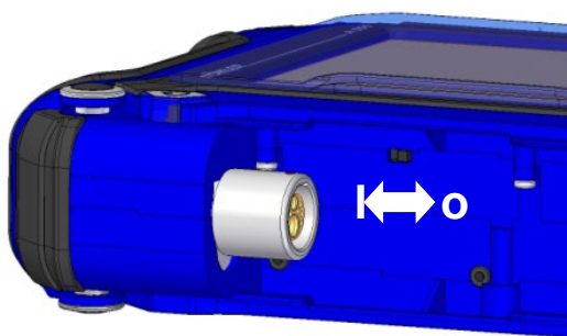
Fig. 21: Push transport lock to the left: batteries activated. Push transport lock to the right: batteries deactivated
