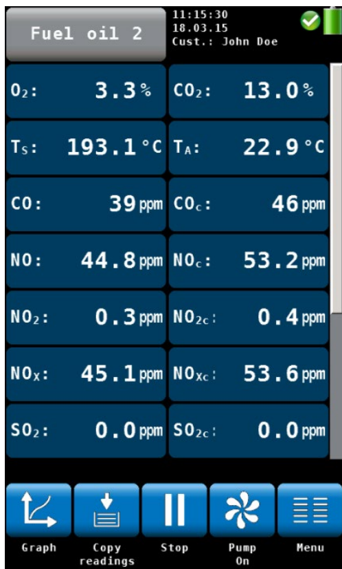
Fig. 18: Display details
