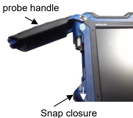
Fig. 20: Wohler A 550 INDUSTRIAL with open probe compartment
