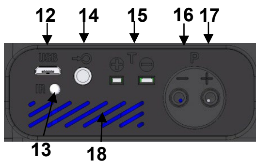
Fig. 6: Connectors at the bottom
