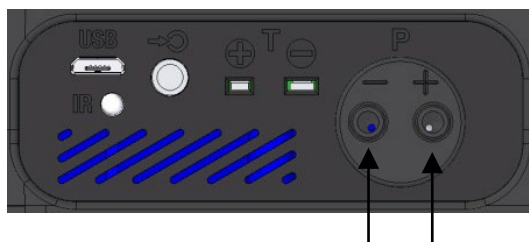
Fig. 55: Negative Pressure Connector at the bottom of the analyzer.
