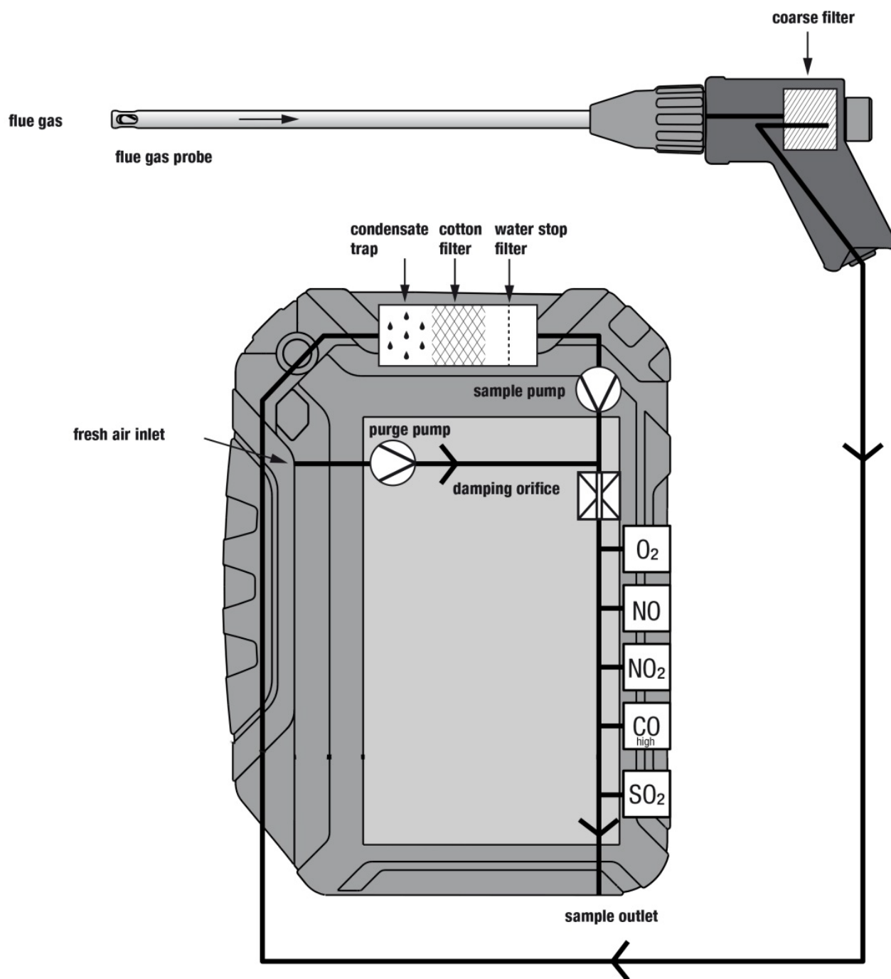
Fig. 19: Gas sampling path Wohler A 550 INDUSTRIAL
