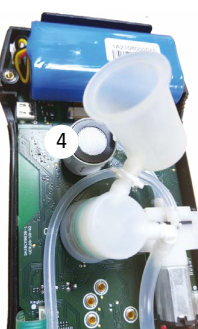
New sensor connected to electronic board
