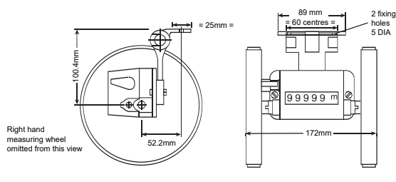
Product Dimensions 2300
