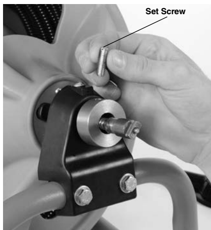
Figure 3 – Remove and discard the Cable Lock Set Screw
