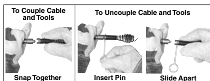
Figure 12 – Connecting/Disconnecting Tools
