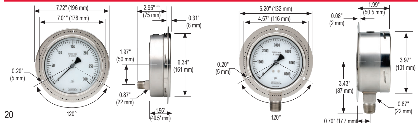
60-410/510 Front Flange
