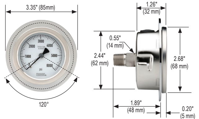
25-410/510 Flange Ring
