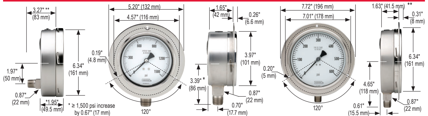
25-410/510 Front Flange
