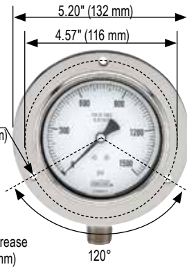
25-410/510 Front Flange
