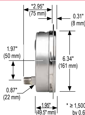
60-410/510 Front Flange
