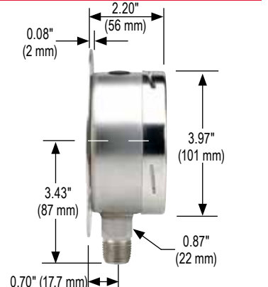
40-400/500 Rear Flange
