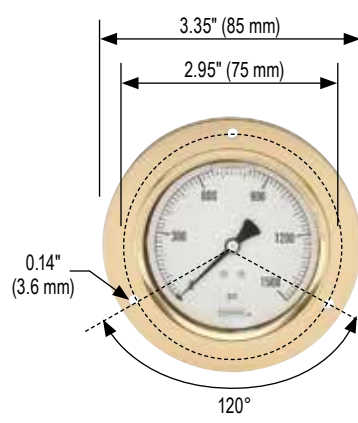
25-310 Front Flange
