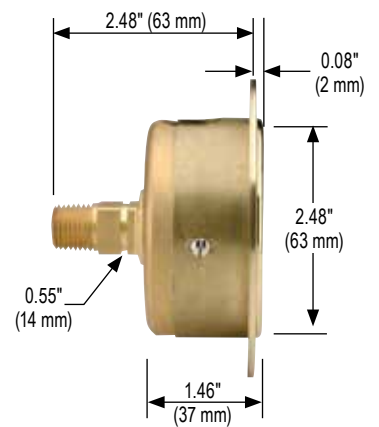
25-310 Front Flange
