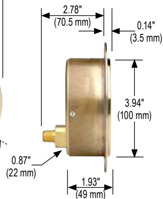
40-310 Front Flange
