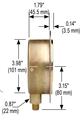
40-300 Front Flange
