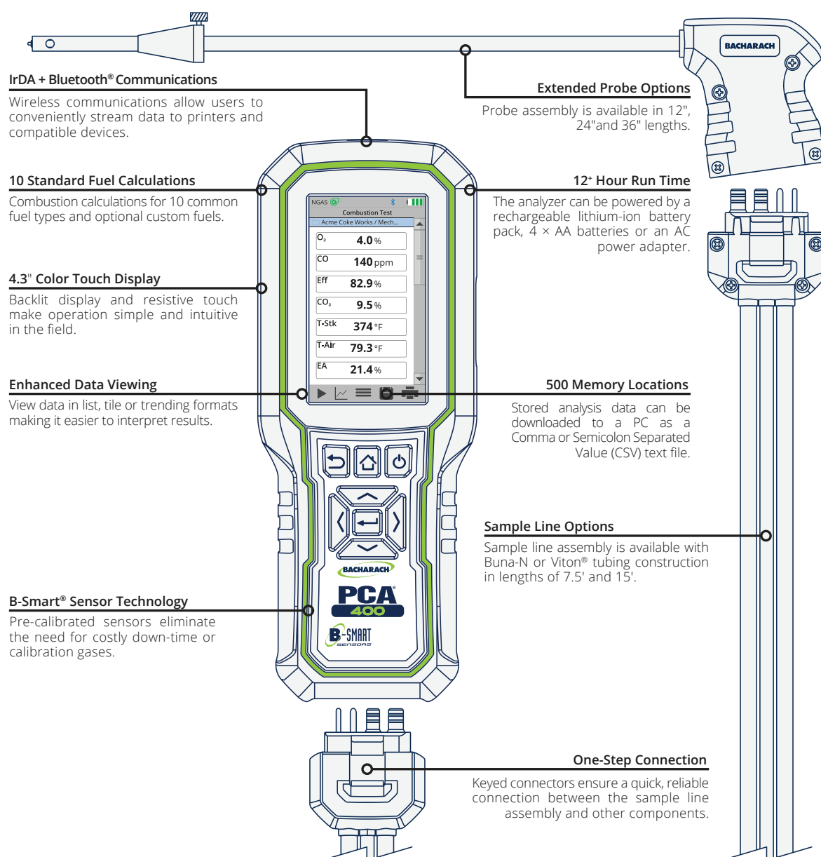
Fig. 2-1: Product Features
