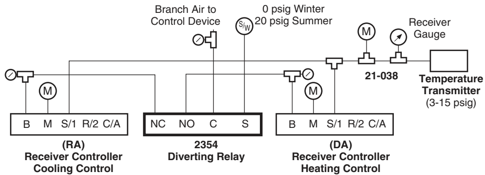
Figure 1 Typical Application.
