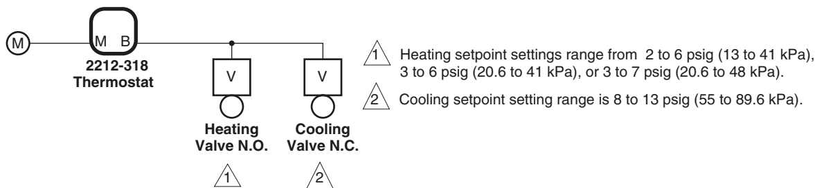
Figure 1 Typical Application.
