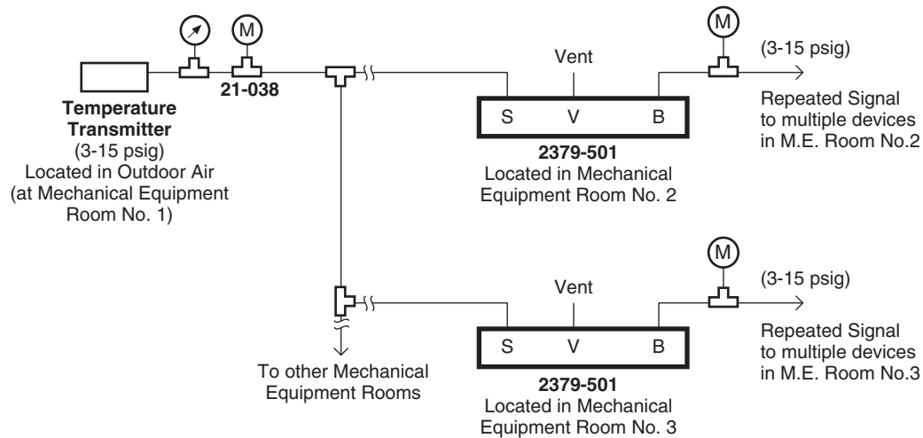
Figure 1 Typical Application.
