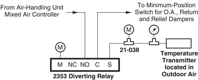
Figure 1 2353-501, 2353-502 Typical Application.
