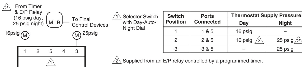
Figure 1 Automatic or Manual Changeover of Day/Night System.
