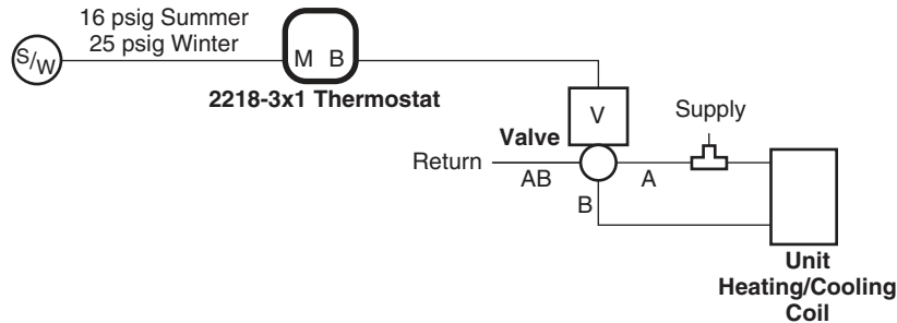
Figure 6 2218-3x1 Typical Application.
