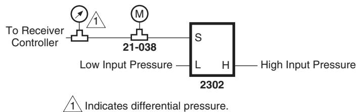
Figure 1 Piping Connections.
