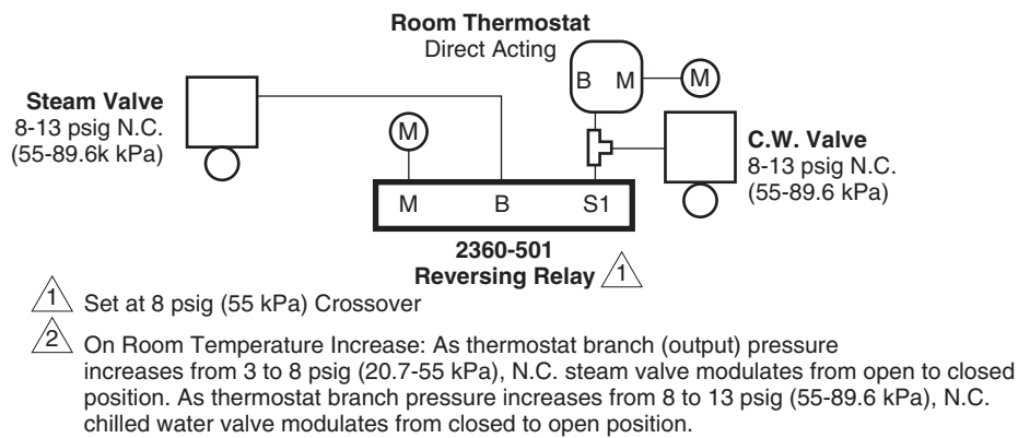
Figure 1 Typical Application.
