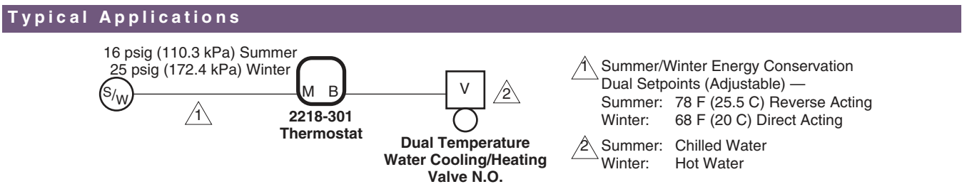
Figure 1 Typical Application.
