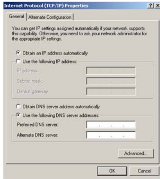
Figure 21 - Properties Dialog
