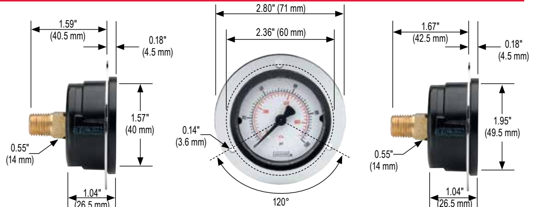
15-110 Front Flange
