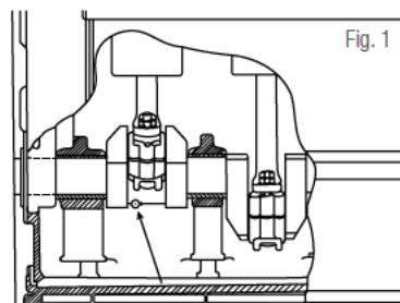
STRAIN GAGE APPLIED TO CRANK OF DIESEL ENGINE TO DETERMINE IMPROPER ALIGNMENT.
