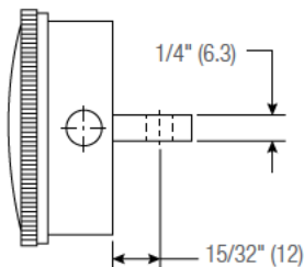
656-129J case stem cap design required for use with lift lever See page 171
