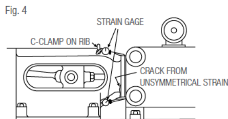
STRAIN BETWEEN APPLIED ENGINE FRAME (WHILE OPERATING), DIFFERENCE BETWEEN TOP AND BOTTOM READINGS OF THE STRAIN GAGE INDICATES IMPROPER ALIGNMENT, CAUSING CRACKS.
