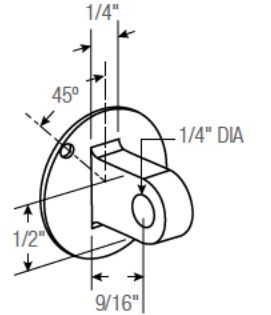
PT25053 Lug-on-Center Back (Standard on all 80 Dial Indicators)
