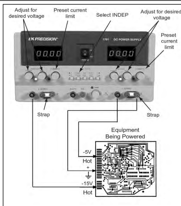
Fig. 14. Typical Hook-Up Using Two Different Negative Voltages and a Common Positive.
