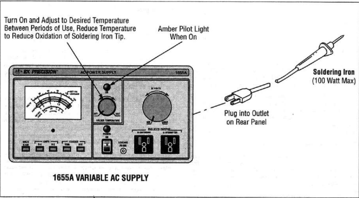
Figure 13. Using the Variable Soldering Iron Temperature Feature.
