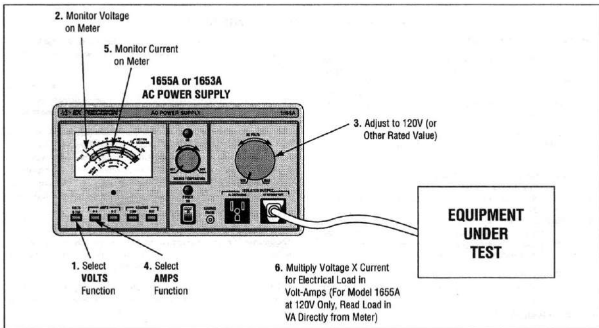
Figure 11. Measuring Electrical Load
