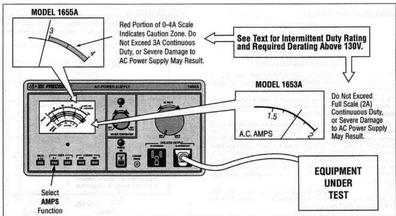
Figure 6. Maximum Current Considerations.
