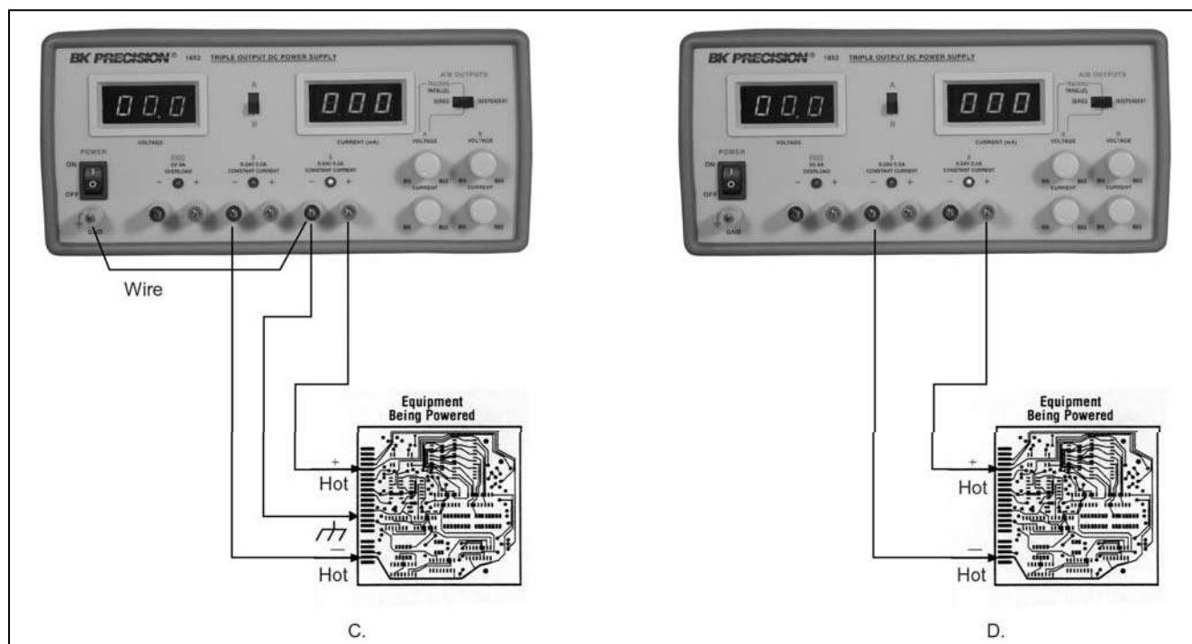
Figure 8. Series tracking (0-48 V) operation grounding possibilities (sheet 2 of 3)
