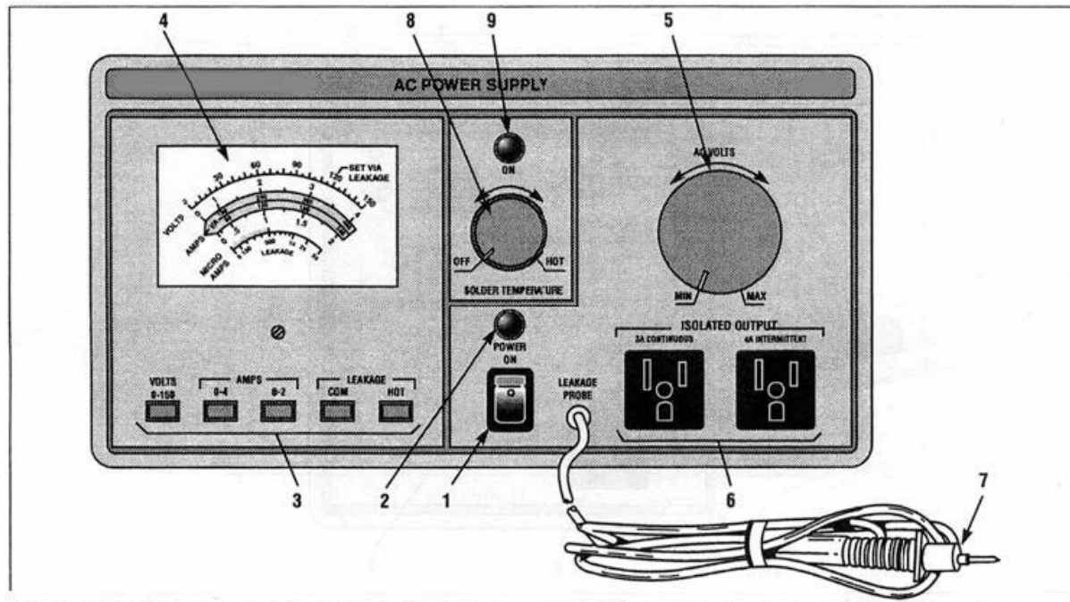
Figure 1. Front Panel Controls and Indicators, Model 1420
