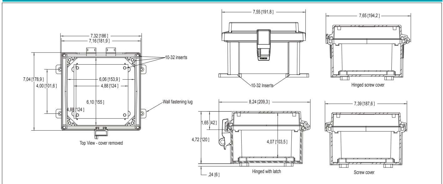
AcuRev 1310 meter installed; AcuRev 1310 meter and AcuRev 1310-ENC are ordered separately.
