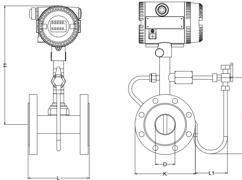
Dimension for Flanged Multi-Variable Type (ANSI 150#)
