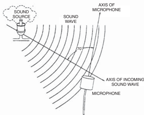
Figure 3-2. Microphone Orientation
