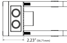
Right View
