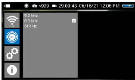
Fig. 32: Locator detection with 8.9 kHz transmission frequency selected
