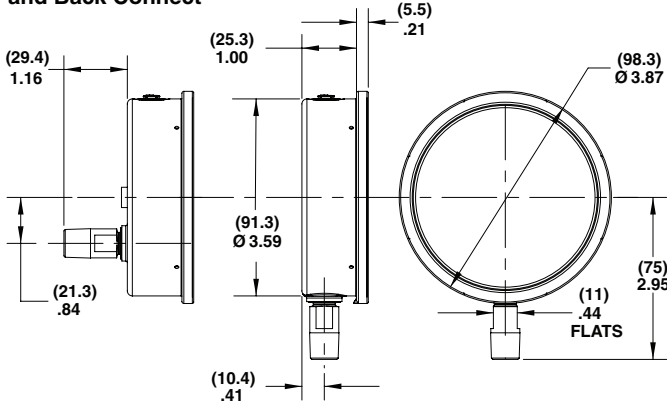
100mm 1008 Lower and Back Connect
