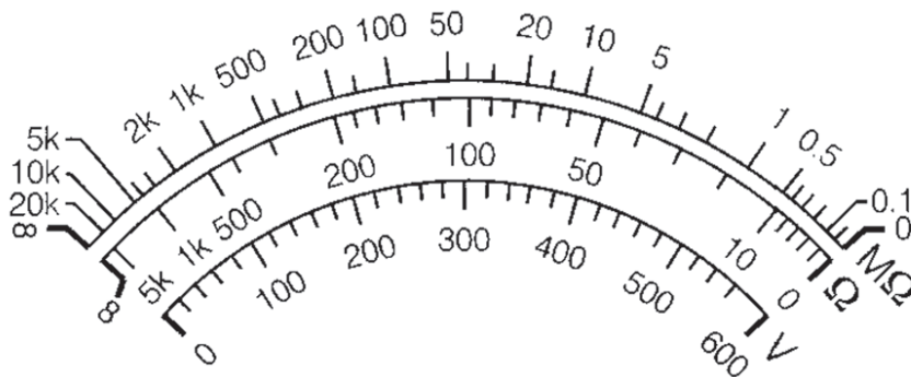
Figure 3—Typical scale on the Megger insulation tester.
