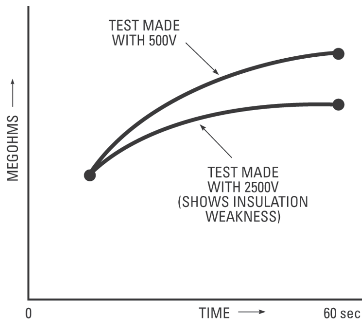
Figure 23-Typical curves with the "step-voltage" test.
