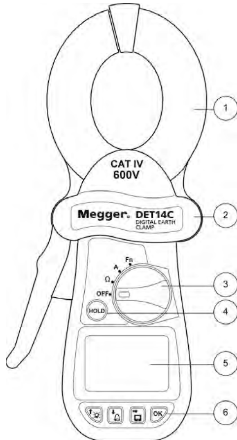
Figure 1: DET14C / DET24C Instrument Front View
