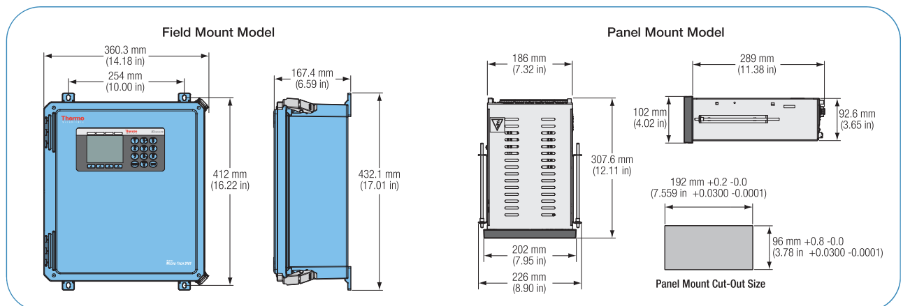
Dimensional drawings for Thermo Scientific Ramsey Micro-Tech 9101 belt conveyor scale integrators
