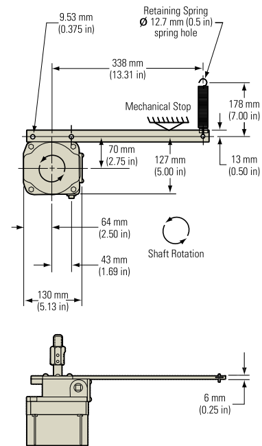
Ramsey 60-12 Speed Sensor
