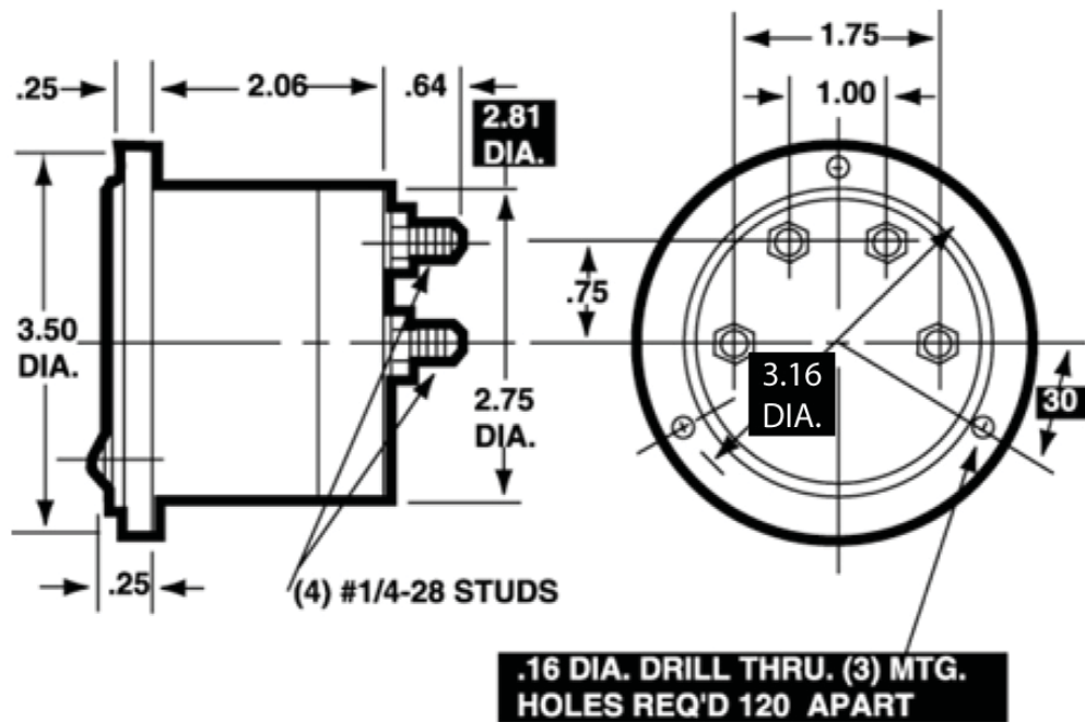
3 - 1/2" Model 75 Wattmeter
