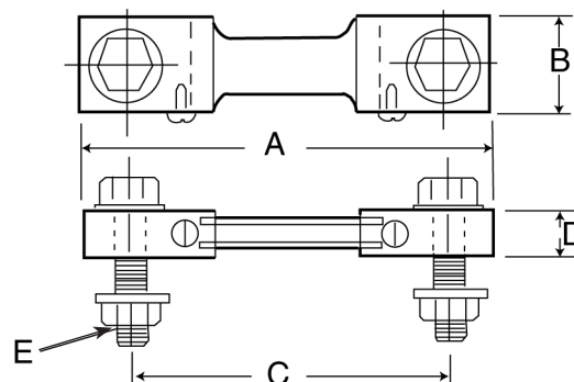
Switchboard Shunts
