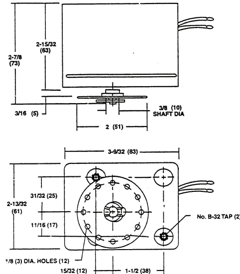
Linkage Drive
