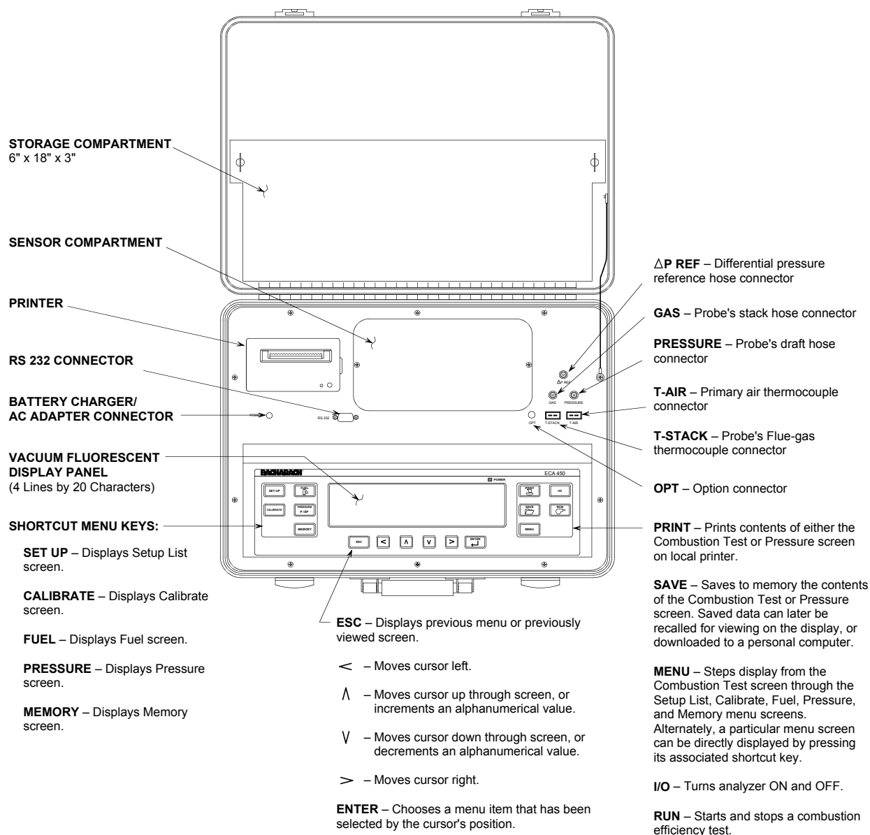
Figure 1-1. ECA 450 Components
