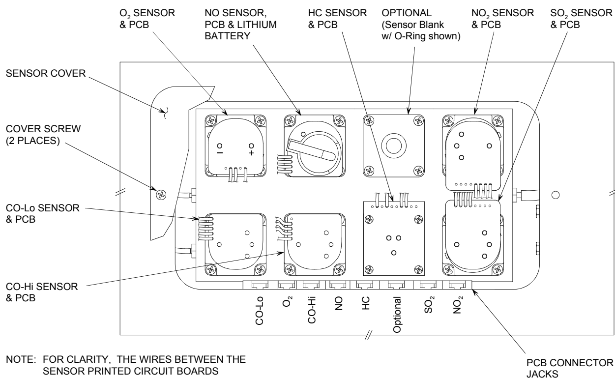
Figure 4-3. Sensor Compartment
