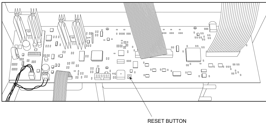
Figure 4-6. Reset Button
