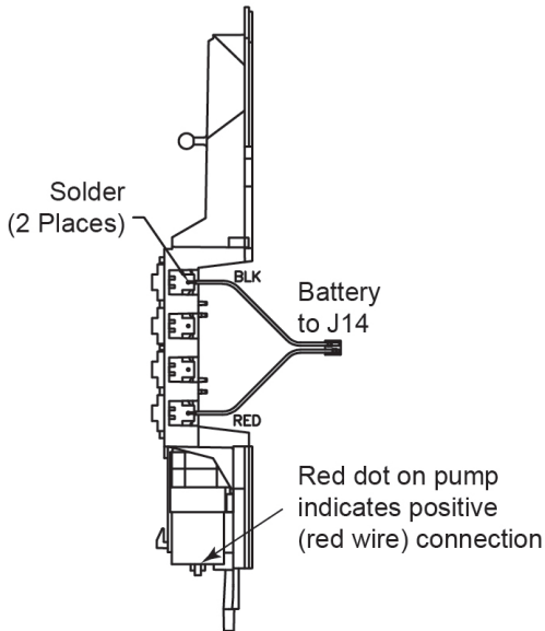
Solder Connections
