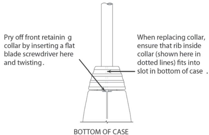
Figure 6. Front Retaining Collar Installation
