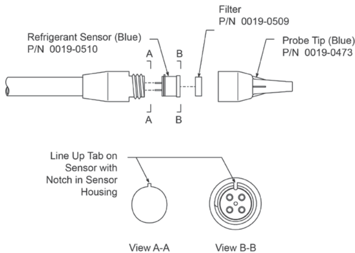
Figure 3a. Sensor Installation (Refrigerant Sensor)
